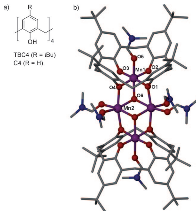
Figure 1. a) Structure of the calix[4]arenes used herein for SMM formation. b) Single-crystal X-ray structure of 1 . Mn purple, O red, N blue, C gray. Hydrogen atoms are omitted for clarity.
